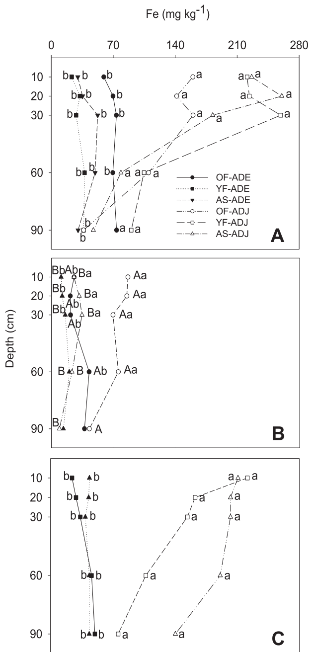
Fig. 3. Availability of Fe (mg kg -1 ) in Amazonian Dark Earths (ADE) and adjacent soil (ADJ) in different land use systems in Iranduba, AM (A), Belterra, PA (B), and Porto Velho, RO (C). OF-ADE = old forest on ADE soil; YF-ADE = Young forest on ADE; AS = Agricultural system on ADE; OF-ADJ = old forest on ADJ soil; YF-ADJ = young forest on ADJ soil; AS-ADJ = agricultural system on ADJ. Different lower-case letters indicate significant differences between ADE and ADJ soils within each land use system, while different upper-case letter indicate significant differences between the land uses (OF, YF, ADJ) within each soil type.
