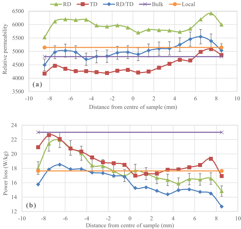
Fig. 4. Local properties, (a) relative permeability and (b) power loss calculated from local H and B measurements for 20 mm wide (160 mm ID) 3.2% SiFe NOES sample. ID edge at -10 mm and OD edge at 10 mm. Measurements taken at a bulk flux density of 1.0 T 400 Hz. Local is the mean value of local measurements. Bulk is the value obtained from the secondary coil and magnetising current.
