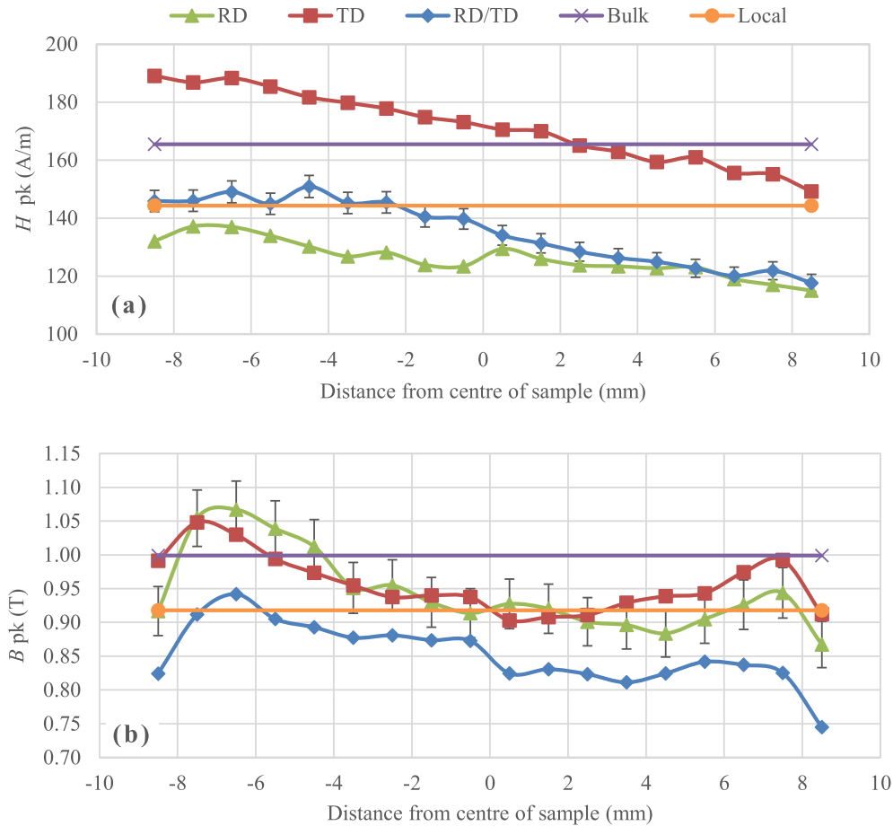
Fig. 3. Local properties, (a) magnetising field and (b) flux density for 20 mm wide (160 mm ID) 3.2% SiFe NOES sample. ID edge at -10 mm and OD edge at 10 mm. Measurements taken at a bulk flux density of 1.0 T 400 Hz. Local is the mean value of local measurements. Bulk is the value obtained from the secondary coil and magnetising current.
