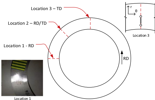
Fig. 2. Schematic of ring sample. The three locations at which measurements were taken were orientated in relation to the rolling direction.
