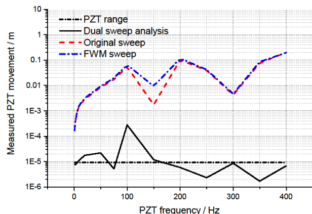
Figure 6. Evolution of the degradation of the single sweep measurements vs frequency for PZT amplitude range of 9 \mu\text{m} .
