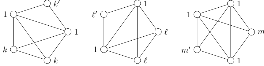
FIGURE 2. Three projections needed for Proposition 31 (1)
