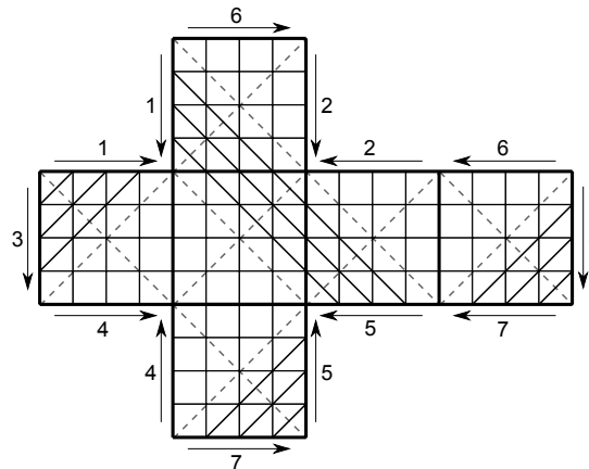
Fig. 4: Identities required to represent a chessboard on a cube as a net, for n even
