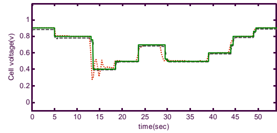
Figure 4. The responses of cell voltage Using a Fuzzy-PID hybrid controller (Ref — Hybrid Control — — mfc .....)
