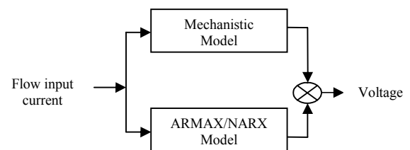
Figure. 6. Hybrid model structure
